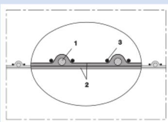
Neoprene hose, double-layer (up to +150°C)
